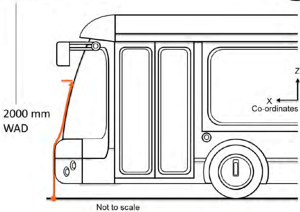
Figure 39_2: Wrap around distance measurement
