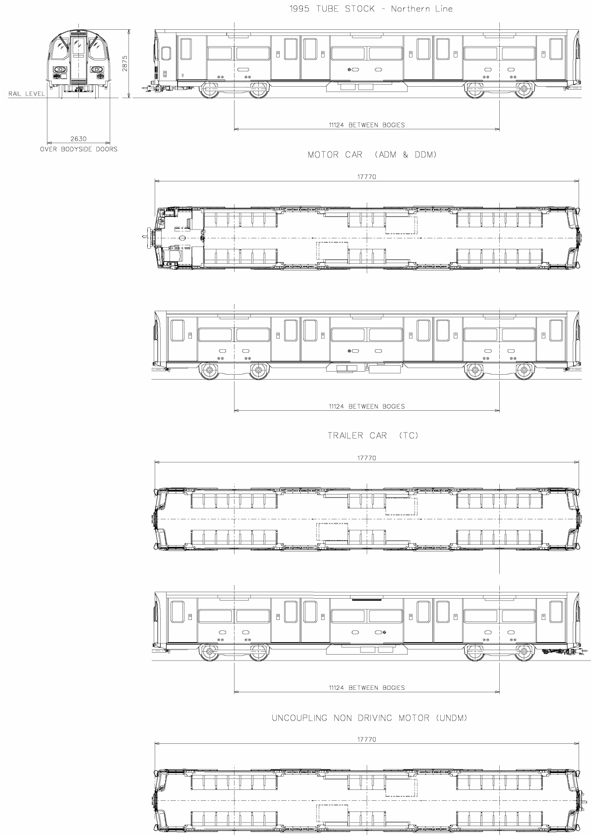
1995 TUBE STOCK - TARE WEIGHT - 156.66 TONNES - 6 CAR TRAIN
