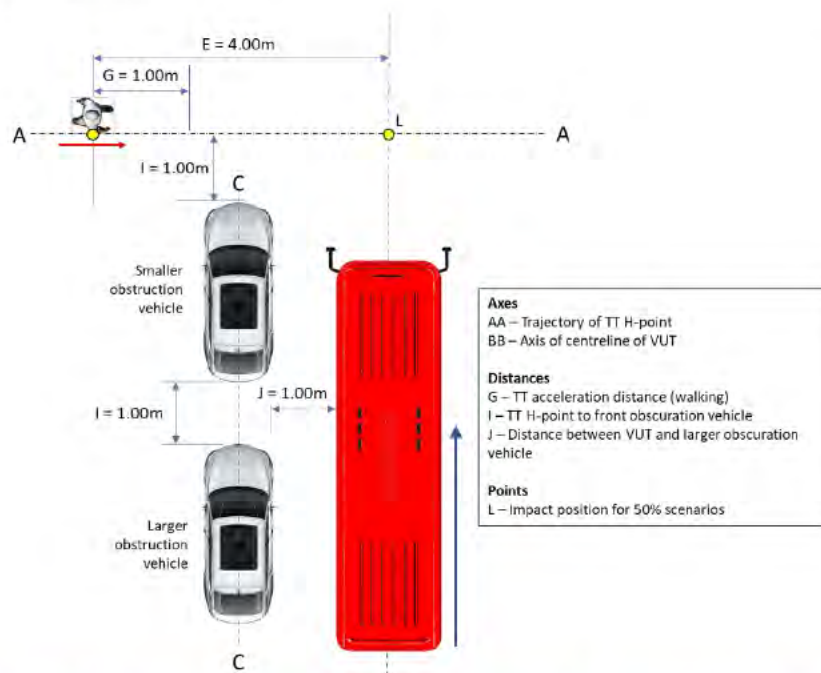
Figure 8: BPNC-50 scenario, child running from the nearside from behind obstructing vehicles
