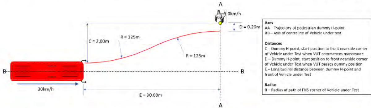
Figure 11: VUT Path and pedestrian position in false positive bus stop test
