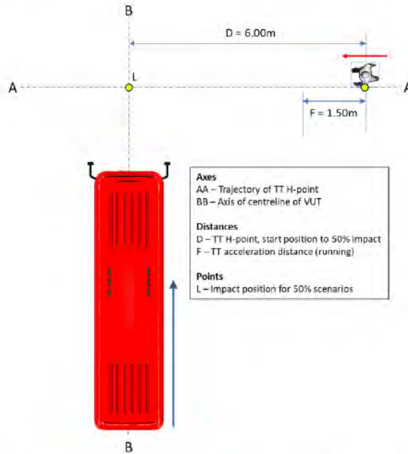
Figure 6: BPFA-50 scenario, adult running from the farside of the road
