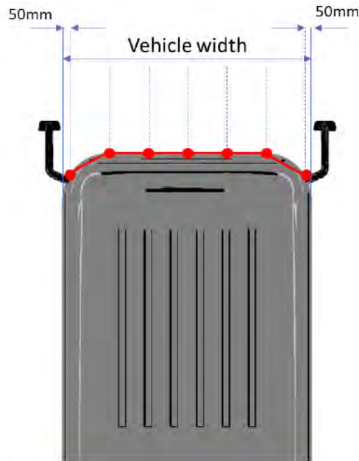
Figure 2: Virtual profile for determining impact for VUT
