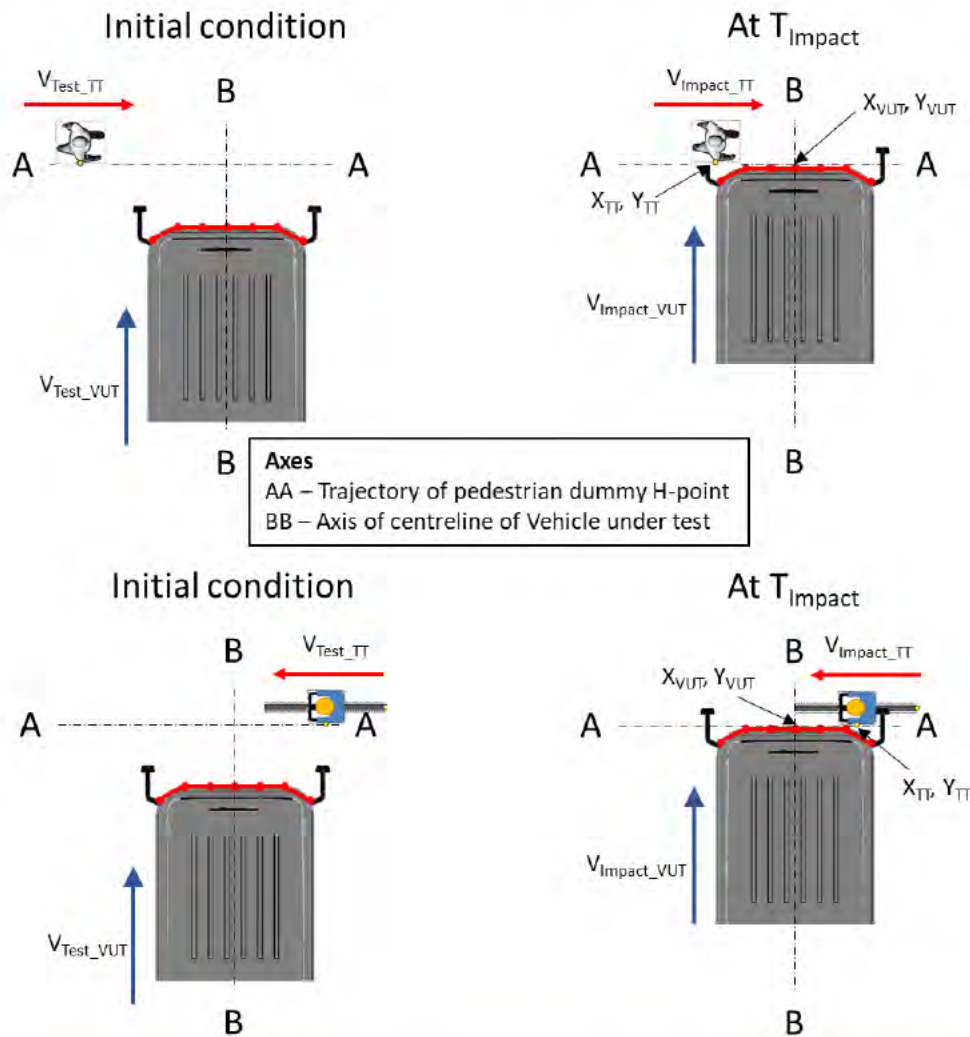
Figure 1: Illustration of the definition of the moment of impact (Pedestrian (top), Cyclist (bottom))
