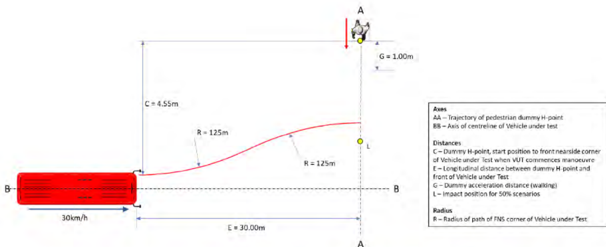
Figure 12: VUT path and TT position in true positive bus stop test
