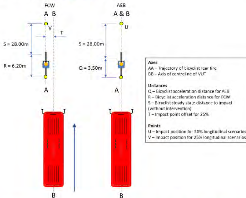
Figure 9: Longitudinal bicyclist scenarios; BBLA-25 (left) & BBLA-50 (right)
