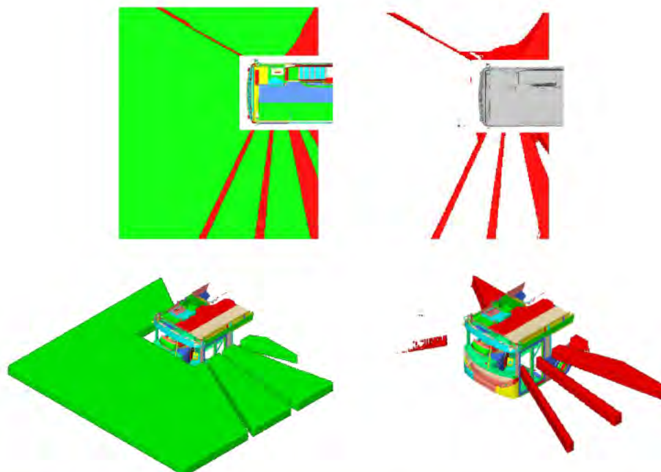
Figure 13: Example images showing Direct Vision Volume (green) and Blind Spot Volume (red) for the forward close proximity assessment zone
