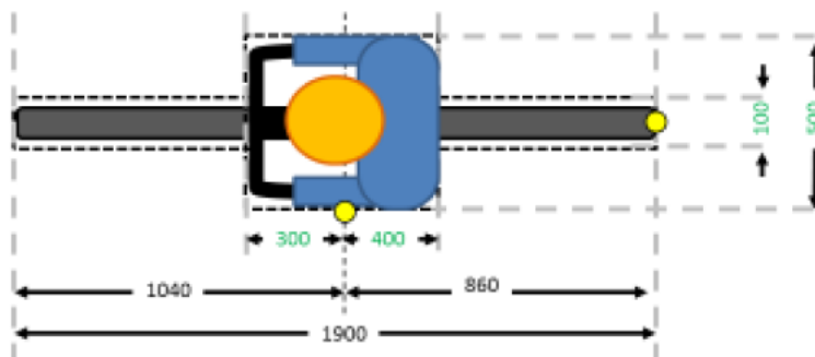
Figure 4: Virtual box around EBT
