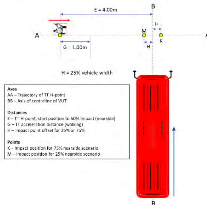
Figure 7: BPNA-25 & BPNA-75 scenario, adult walking from the nearside of the road
