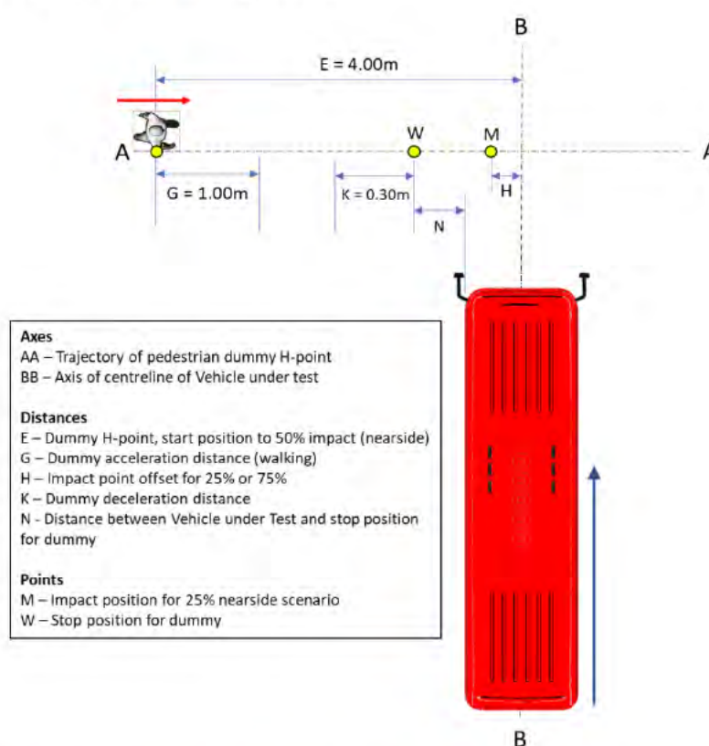
Figure 10: TT start and stop positions in aborted crossing test
