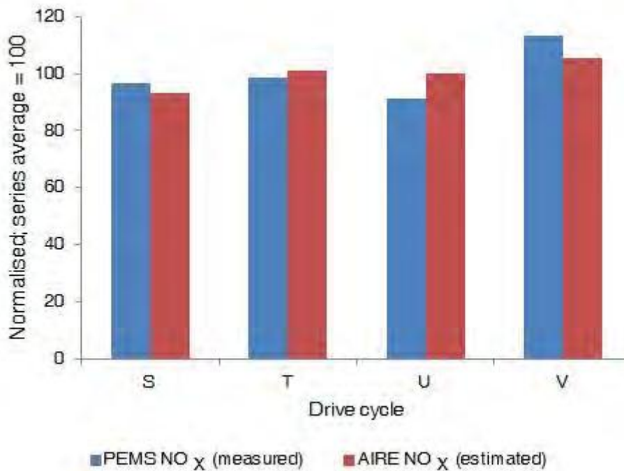
Figure 33: Measured and modelled NO x emissions (constrained, normalised)
