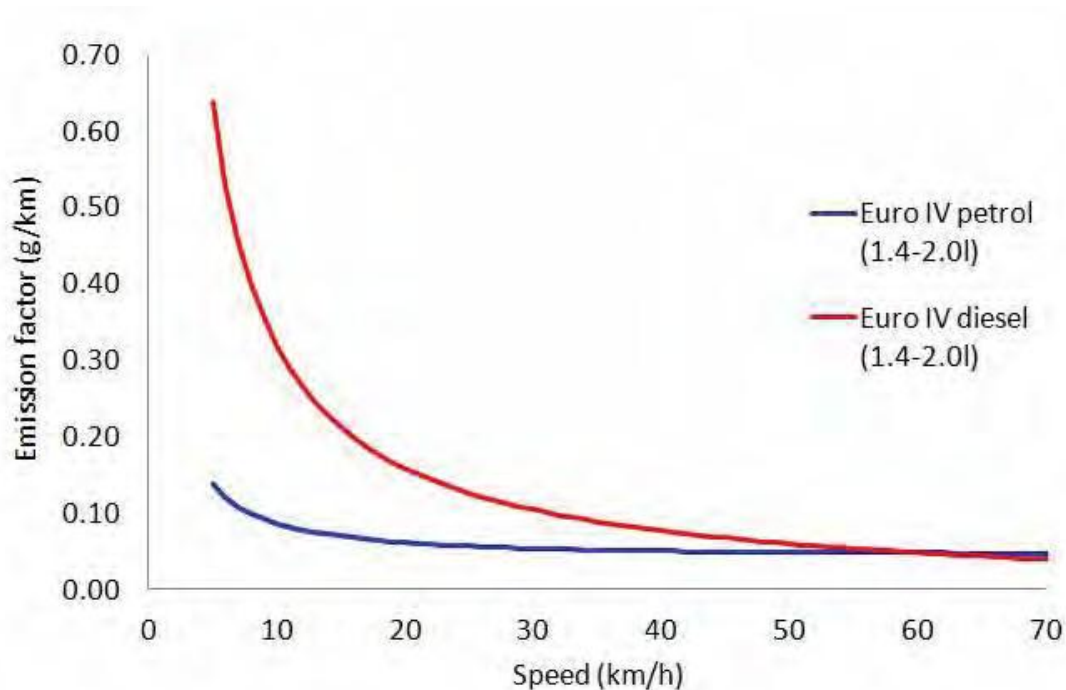
Figure 28: Vehicle emission curve for NO x [generated from 15]
